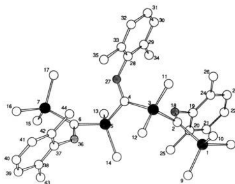
Figure 1. Crystal structure of 3g . Hydrogen atoms have been omitted for clarity. Some bond distances (Å) and angles (deg) are as follows: Si(1)-C(2) = 1.90 (1), C(2)-Si(3) = 1.94 (1), Si(3)-C(4) = 1.92 (1), C(4)-Si(5) = 1.88 (1), Si(5)-C(6) = 1.87 (1), C(6)-Si(7) = 1.91 (1), C(2)-N(18) = 1.27 (1), C(4)-N(27) = 1.30 (1), C(6)-N(36) = 1.32 (1); Si(1)-C(2)-N(18) = 128.2 (8), Si(3)-C(2)-N(18) = 109.6 (8), Si(3)-C(4)-N(27) = 126.0 (8), Si(5)-C(4)-N(27) = 109.6 (8), Si(5)-C(6)-N(36) = 109.1 (8), Si(7)-C(6)-N(36) = 123.4 (8).
