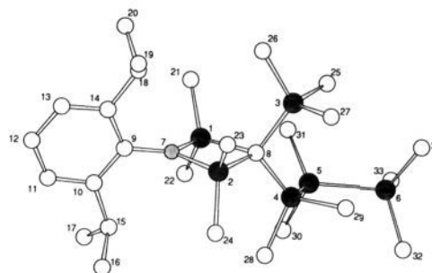
Figure 2. Crystal structure of 18h . Hydrogen atoms have been omitted for clarity. Some bond distances (Å) and angles (deg) are as follows: Si(1)–N(7) = 1.738 (3), Si(1)–C(8) = 1.907 (4), Si(2)–N(7) = 1.734 (3), Si(2)–C(8) = 1.909 (4), N(7)–C(9) = 1.446 (5); Si(1)–C(8)–Si(2) = 84.9 (2), Si(1)–N(7)–Si(2) = 95.8 (2), N(7)–Si(1)–C(8) = 89.4 (2), N(7)–Si(2)–C(8) = 89.4 (2).
